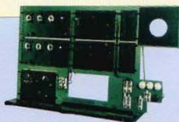
1933-35 Radar
